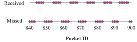
Fig. 8. Received packet sequence.
