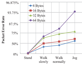
Fig. 6. Packet error rate for different sized packets under various speeds ( y -axis in log scale).
