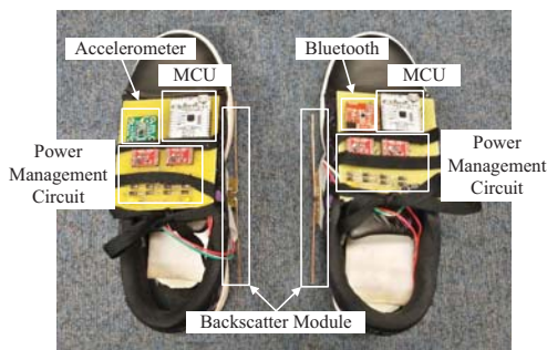
Fig. 9. Pictures of our prototype.
