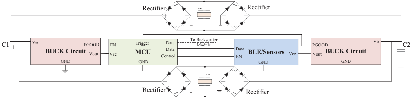
Fig. 5. Circuit diagram.
