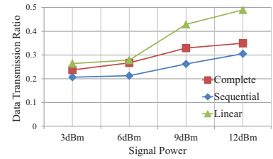
Fig. 12. Different signal power.
